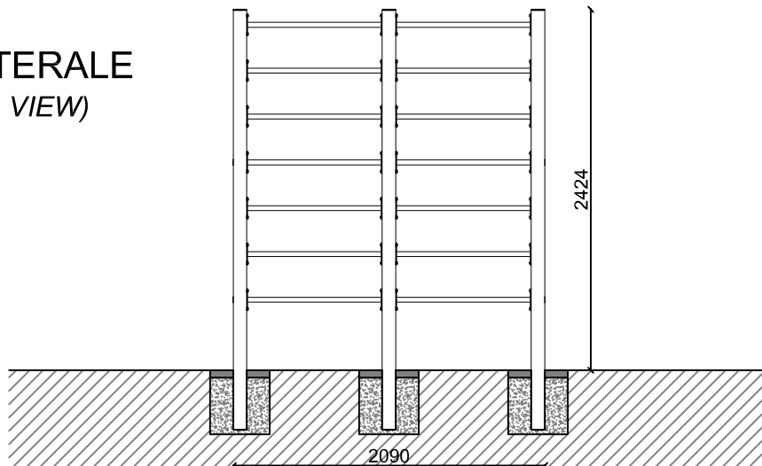
INGOMBRO MAX (OVERALL DIMENSIONS)
